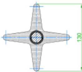
Image 12. Star shed scheme for 300020 code
