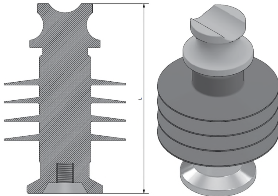
Image Line post insulators
