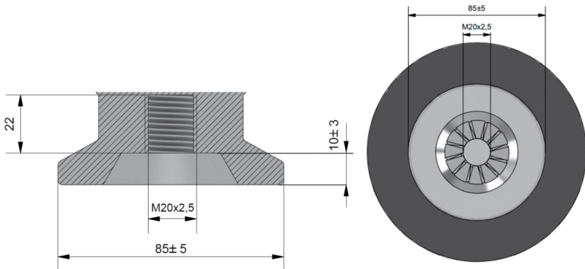
Image 8.2. Base for line post insulators
