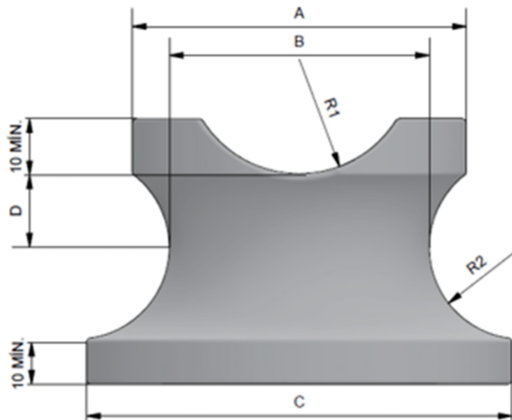
Image 8.1. Fittings for line post insulators
